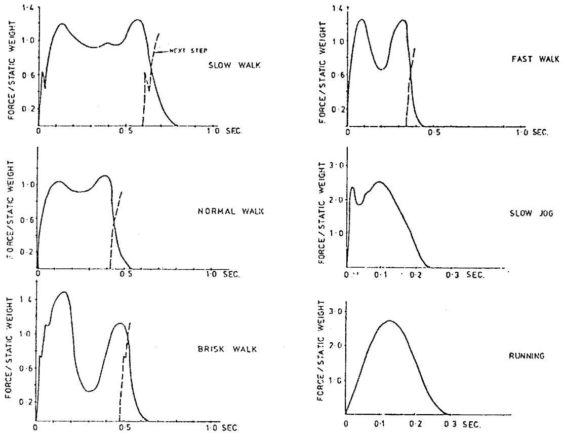
FIG. 1.—Pedestrian Force-Time Histories
